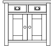
SMALL SIDEBOARD H 773 W: 840 D: 350
