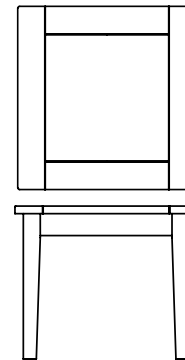
3' x 3' FLIP TOP EXTENDING TABLE H 780 W: 915-1830 D: 915
