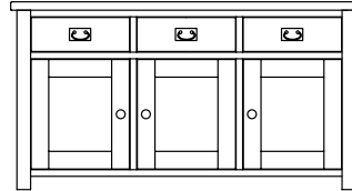
LARGE SIDEBOARD H 850 W: 1590 D: 425
