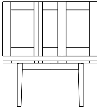
4' EXTENDING TABLE (1 LEAF) H 778 W: 1200-1600 D: 915
